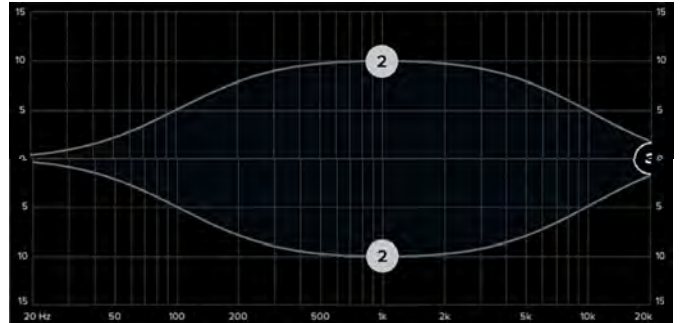
EQ OFF – Mid Band (2) – 1 kHz at ±10 dB
