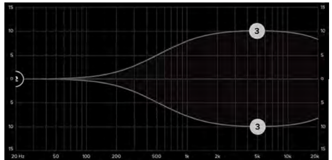
EQ OFF – High Band (3) – 5 kHz at ±10 dB
