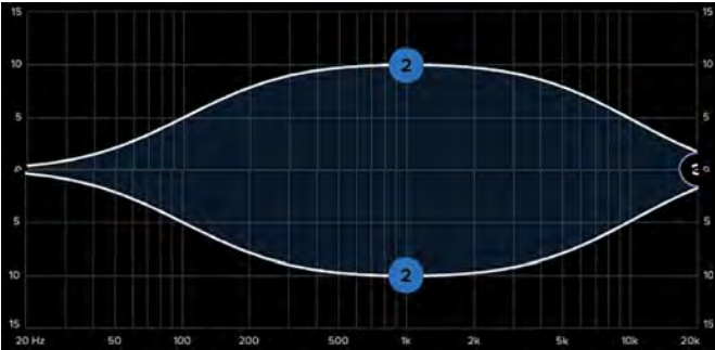
EQ ON – Mid Band (2) – 1 kHz at ±10 dB
