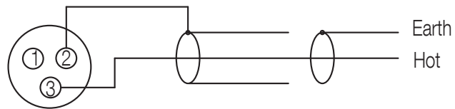
Connection Diagram
