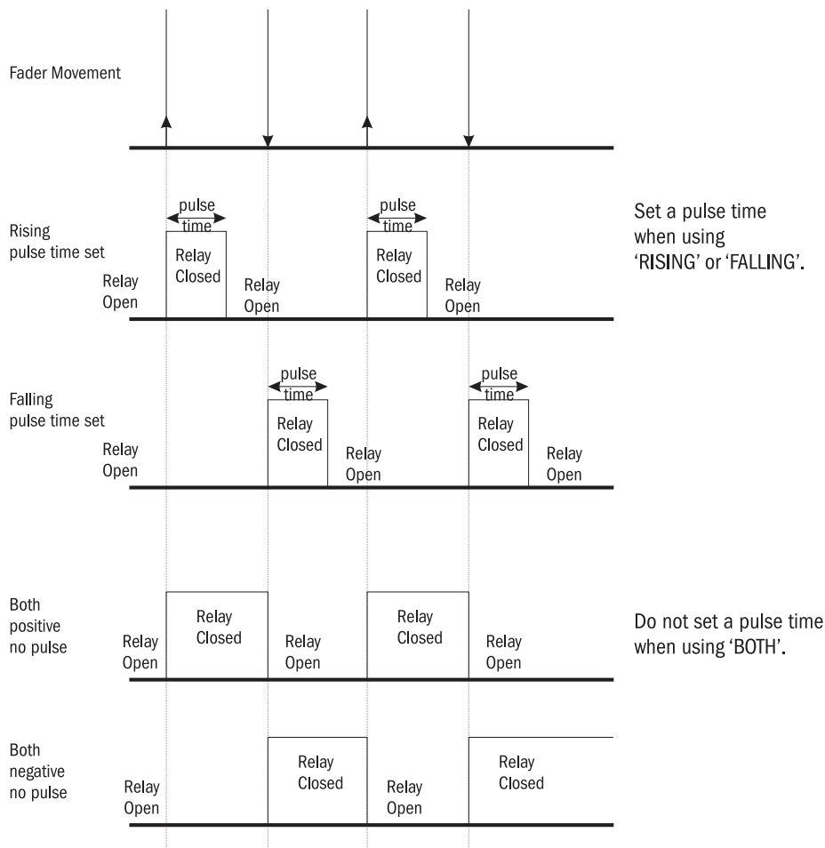
Figure 16-2: Relay timing diagram.
