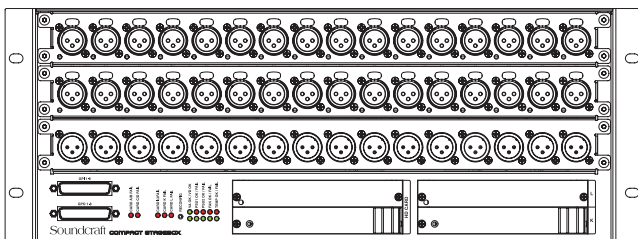
4U Stage Box
