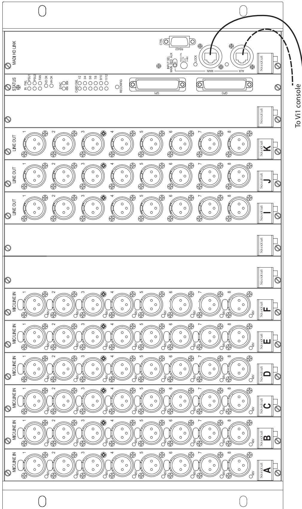
Optional Stage Box (Vi6 type) Front Panel.
