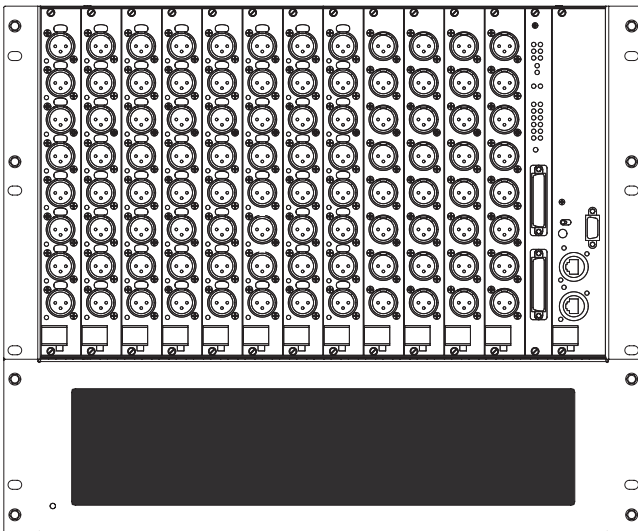
6U Stage Box
