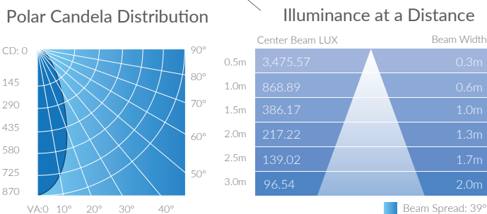
All LEDs On With 40° Diffuser
