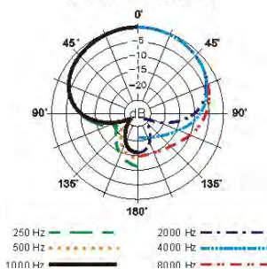
Polar Pattern
