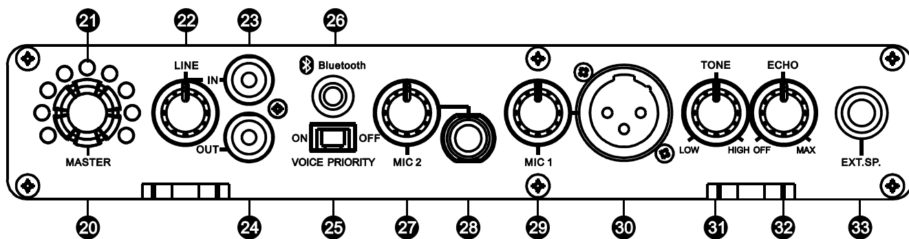
Fig. 3: Control Panel
