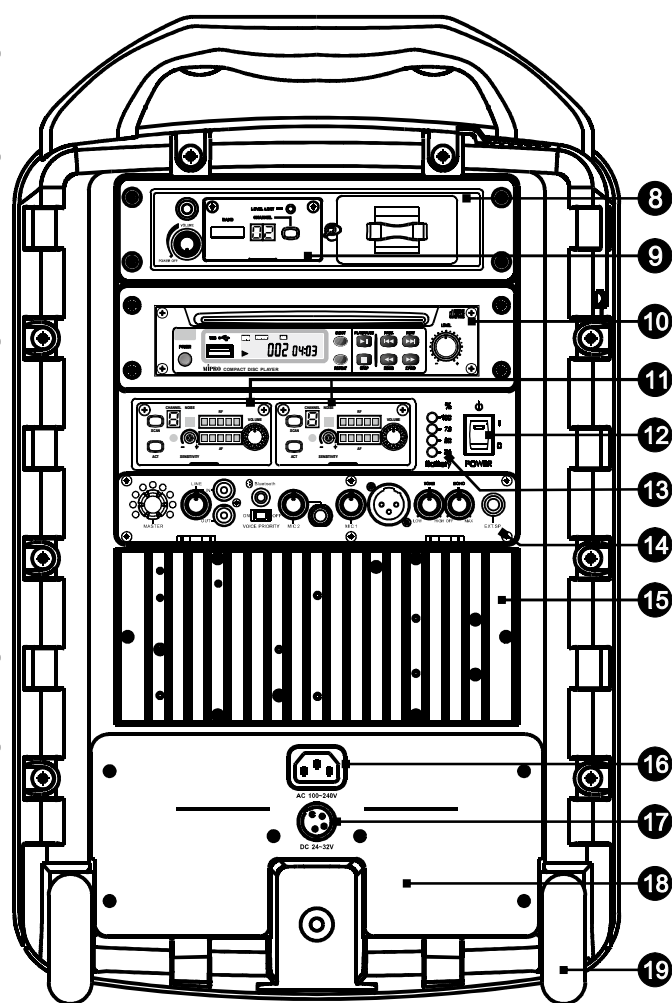
Fig. 2: Rear Panel
