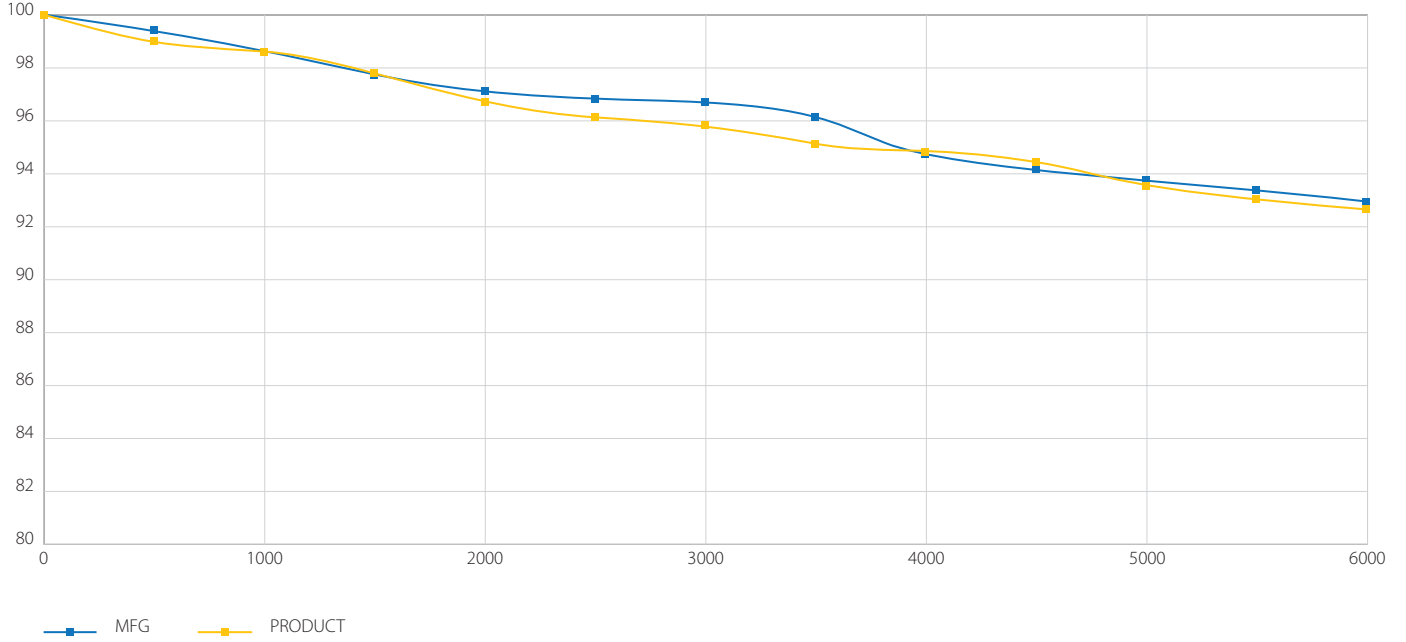
Lumen MFG vs Product 0-6000 Hours
