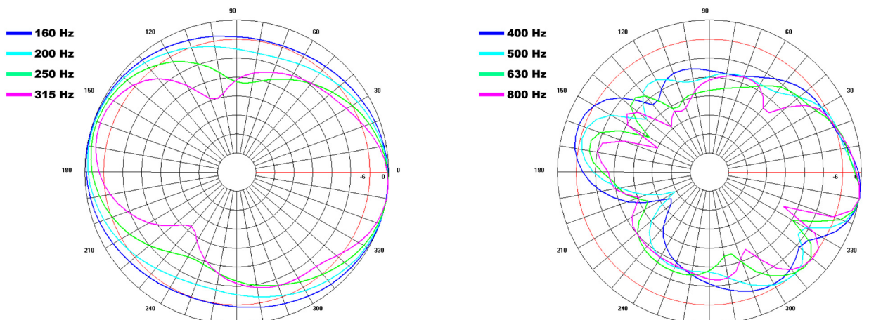
Fig. 8: Horizontally configured PD5322 - modeled vertical polar response
