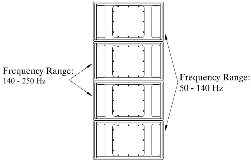
Fig. 9: Four-element PD5122 shaded array
