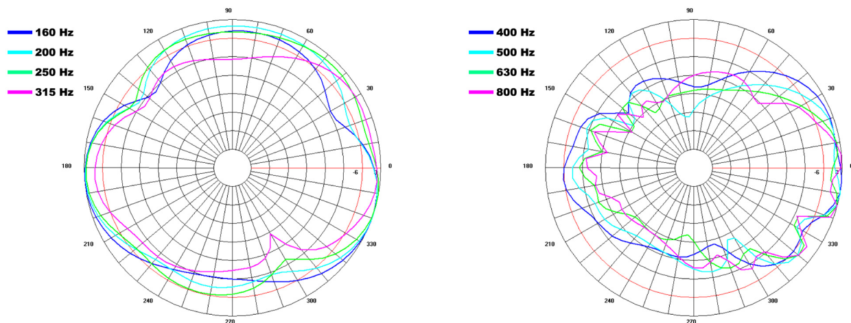
Fig. 5: Vertically configured PD5322s
