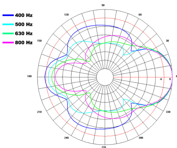
Fig. 3: PD5322 + PD5122 - modeled vertical polar response
