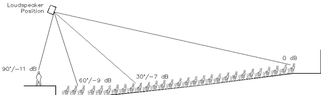
FIG. 1: SECTION
