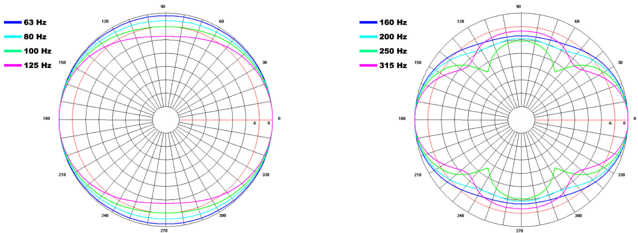
Fig. 10: PD5122 shaded array - modeled vertical polar response
