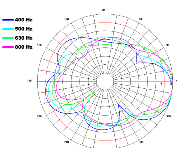
Fig. 4: Steered PD5322 + PD5122 - modeled vertical polar response
