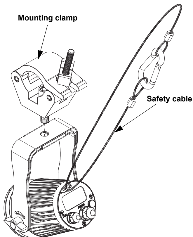
Overhead mounting
