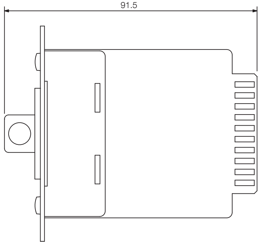
Side View
