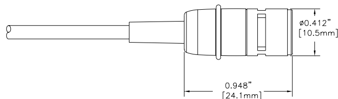
Microphone Dimensions
